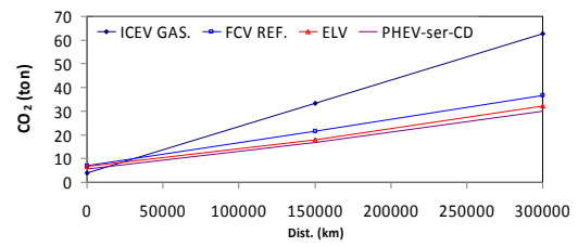
Figure 4: Influence of the distance travelled on full life cycle CO 2 emissions per vehicle.
