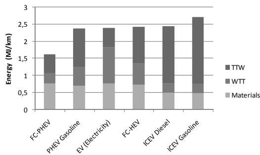
Figure 2: Full life cycle energy for selected vehicles.
