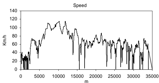
Figure 1: Experimentally measured driving cycle.
