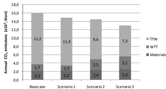
Figure 6: Annual fleet's life cycle results for materials, WTT and TTW regarding CO 2 emissions in the considered scenarios.
