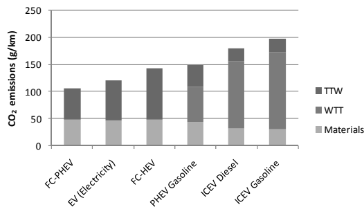
Figure 3: Full life cycle CO 2 for selected vehicles.
