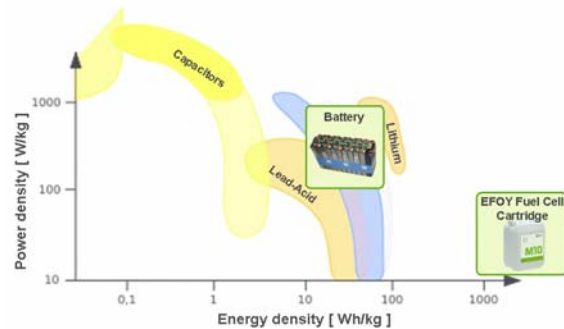
Figure 2: DMFC's superior energy density provides easier handling and greater efficiency
