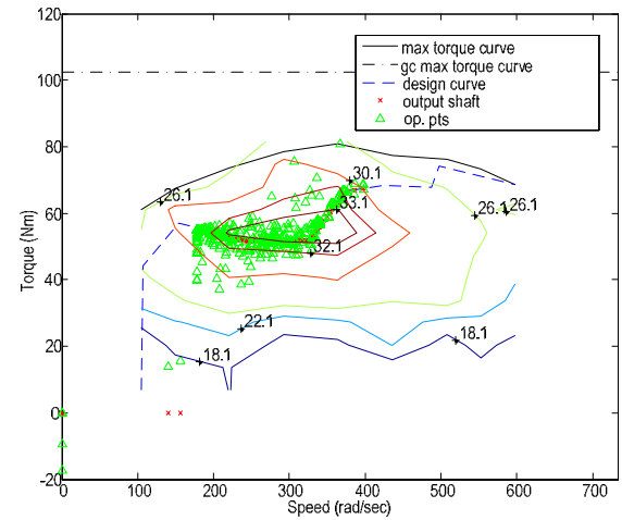
Fig. 5. Engine operation (proposed method)
