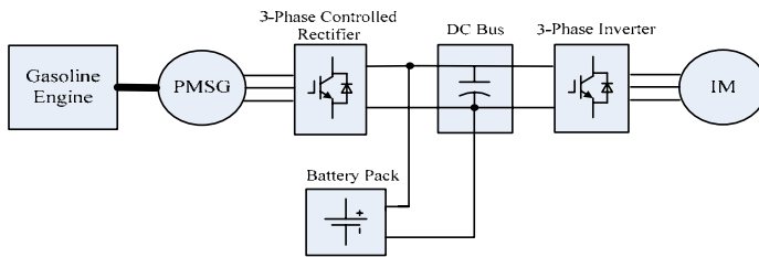
Fig. 1. Powertrain structure of SHEV.
