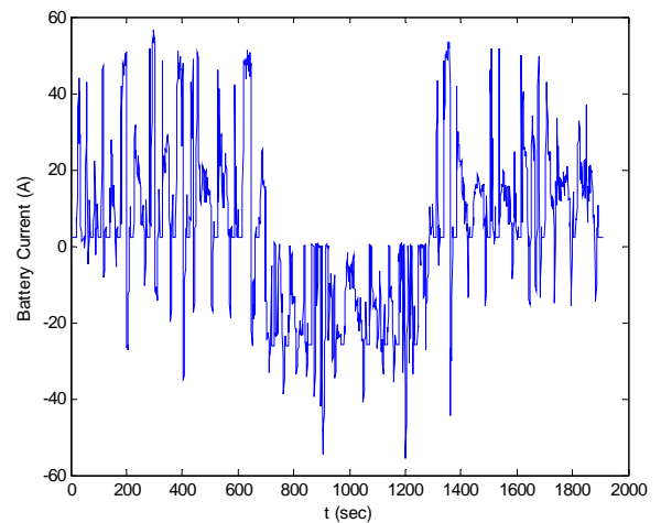
Fig. 6. Battery current during OCC (conventional method).
