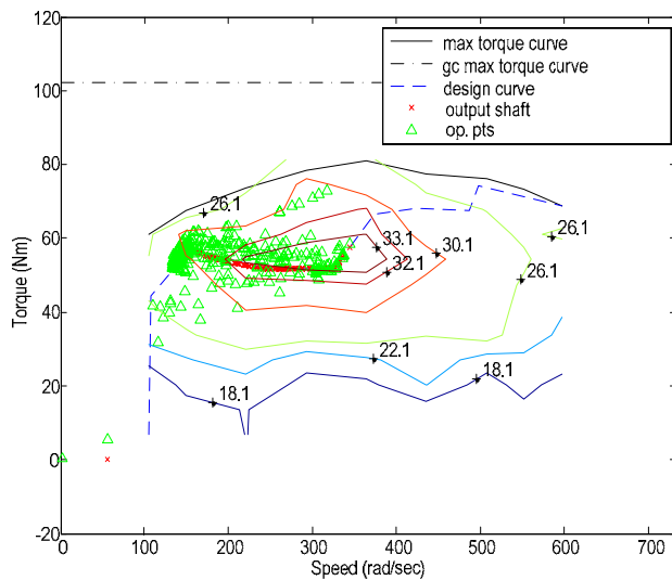
Fig. 4. Engine operation (conventional method).
