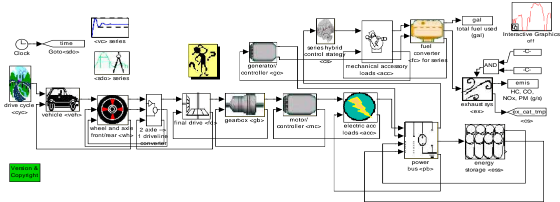
Fig. 3. Modified SHEV model for algorithm implementation
