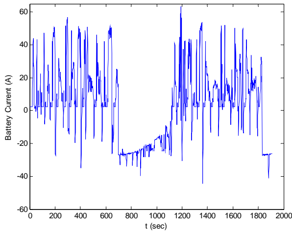
Fig. 7. Battery current during OCC (proposed method).
