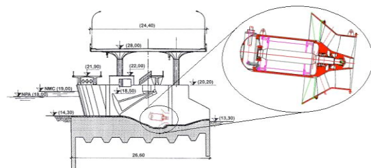
Figure23: Profile view of Coimbra dam-bridge with a turbine-generator unit
