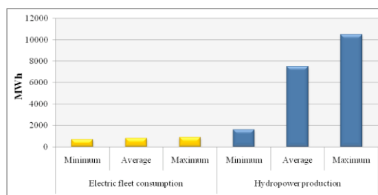
Figure26: Electric fleet consumption and hydropower production
