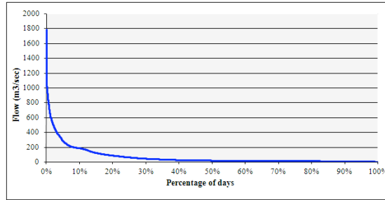
Figure24: Coimbra dam-bridge flow duration curve
