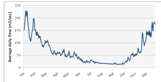
Figure22: Average daily flow
