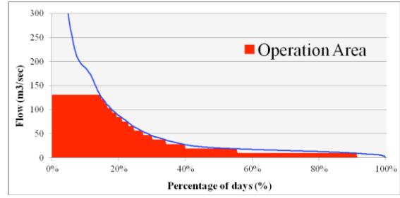
Figure25: Small hydro operation area
