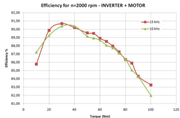
Figure8: Comparison of \eta=f(T) – inverter + motor
