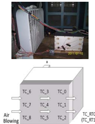
Figure 6: Test setup for the fast charging of the 24V module
