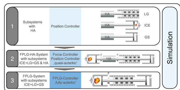
Figure 2: Development methodology for the FPLG
