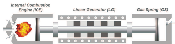
Figure 1: FPLG-system with the three subsystems internal combustion engine, linear generator and gas spring.
