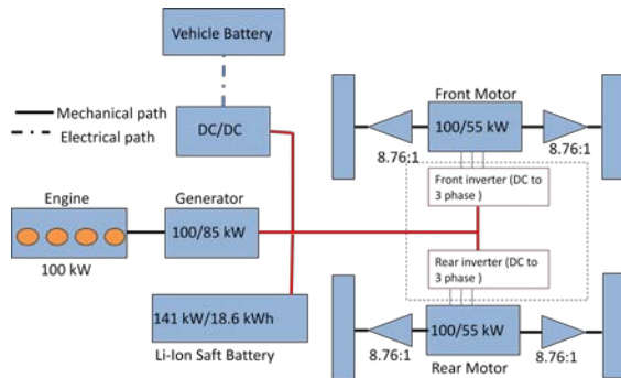
Figure 5: The XM1124 Schematic
