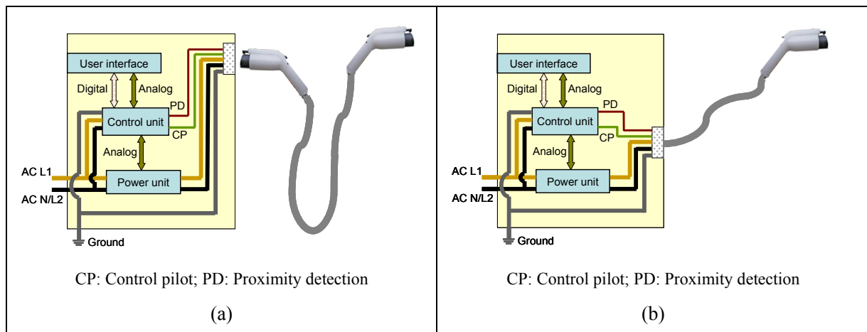
Figure 2: Schematic diagram of major units for an AC charging stand: (a) IEC 61851-1 Case “B” connection; (b) IEC 61851-1 Case “C” connection and SAE J1772
