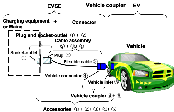
Figure 1: Terminology used in conductive charging system
