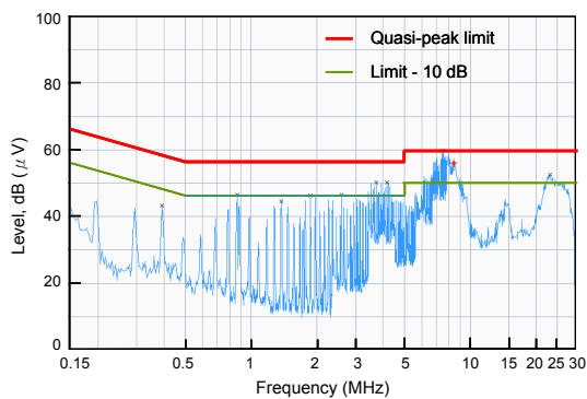
Figure 5: Conducted emission at AC input terminal line 2, operating with 32 A load and deducting the influence of simulator
