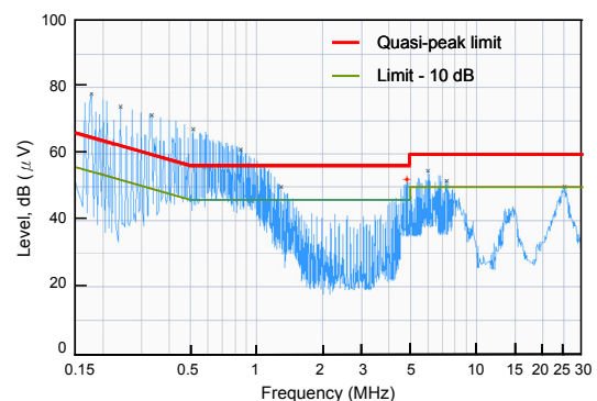
Figure 4: Conducted emission at AC input terminal line 2, operating with 6 A load
