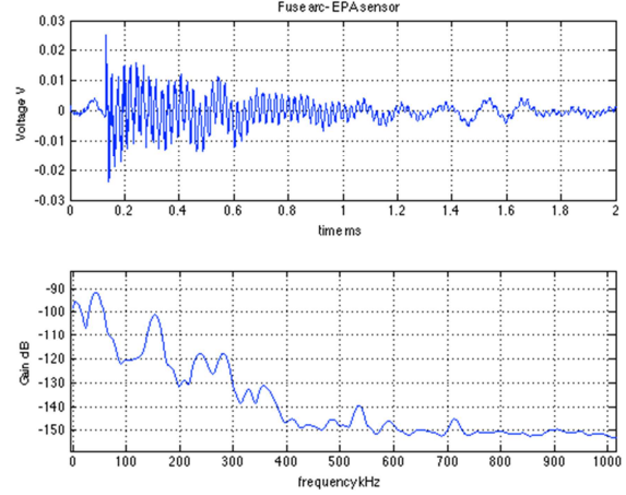
Figure 1: Time and frequency signatures of a fuse arc measured with an EPA sensor.
