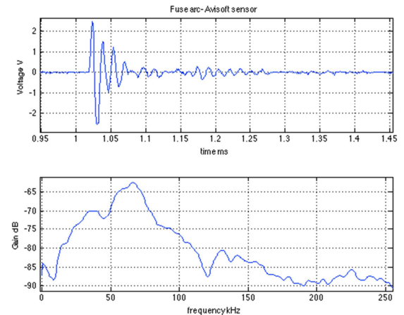
Figure 2: time and frequency signatures of a fuse arc measured with an Avisoft sensor.
