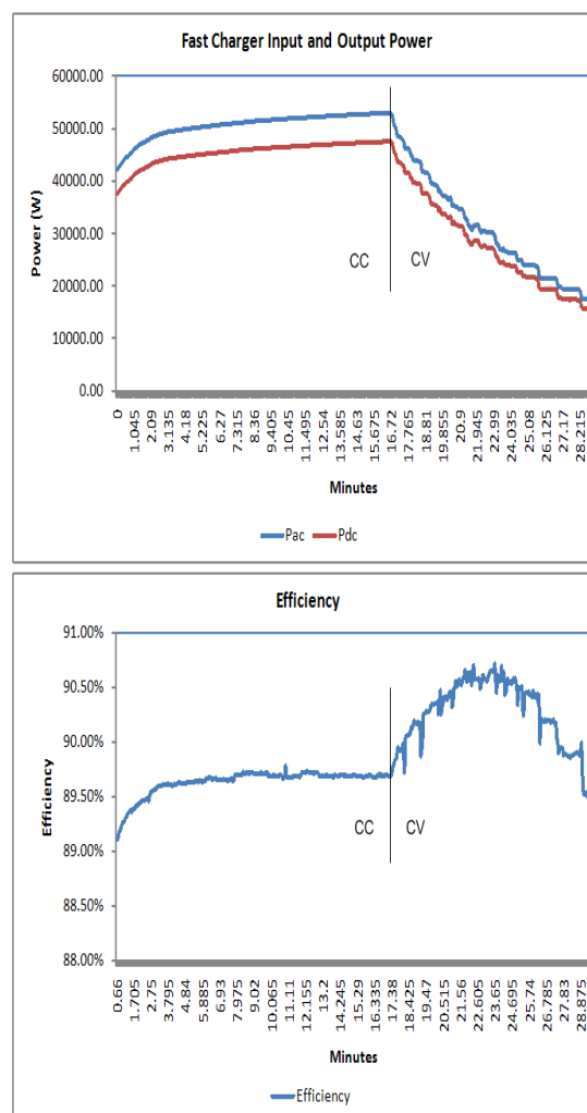
Figure 8: Nissan Leaf Input and Output Power Charge Profile and Associated DC Fast Charger Efficiency
