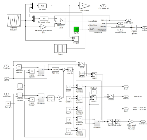
Figure 9: Driving cycle and control logic block
