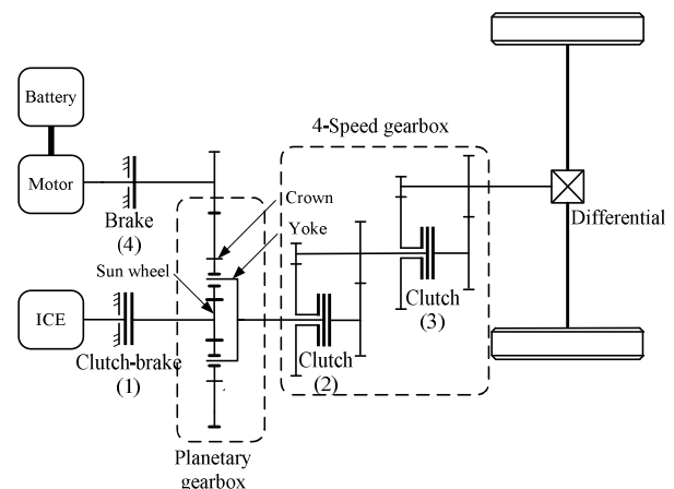
Figure1: Configurations of the improved CHPTD with gearbox
