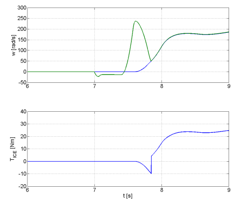
Figure 23: Simulation results of ICE speed, sun shaft speed and ICE torque during ICE starting (No12 in Table 4)
