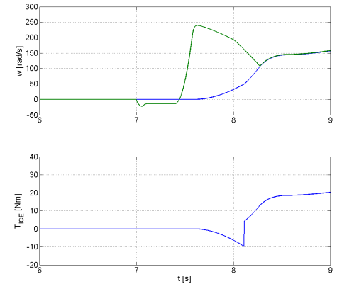
Figure 22: Simulation results of ICE speed, sun shaft speed and ICE torque during ICE starting (No11 in Table 4)
