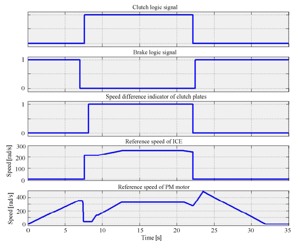
Figure 10: Control signal generated by control logic block
