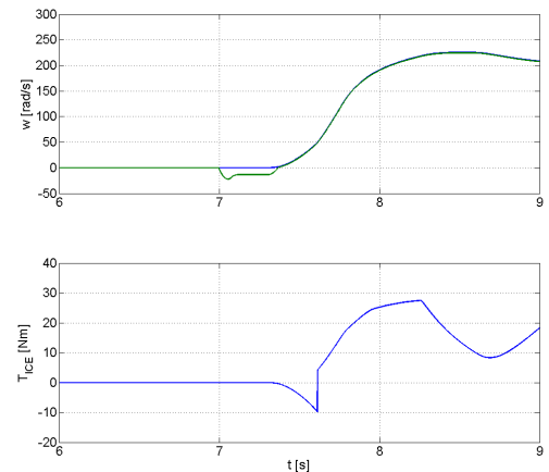
Figure 18: Simulation results of ICE speed, sun shaft speed and ICE torque during ICE starting (No4 in Table 4)
