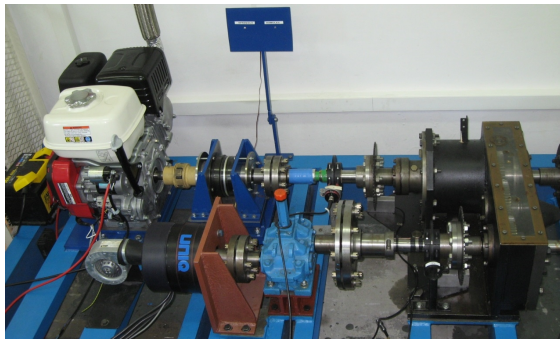
Figure 3: Laboratory stand of CHPTD
