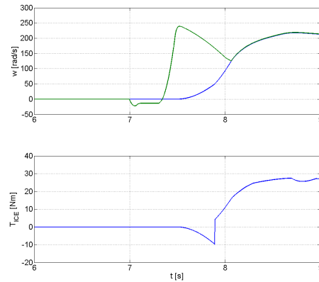
Figure 25: Simulation results of ICE speed, sun shaft speed and ICE torque during ICE starting (No6 in Table 4)
