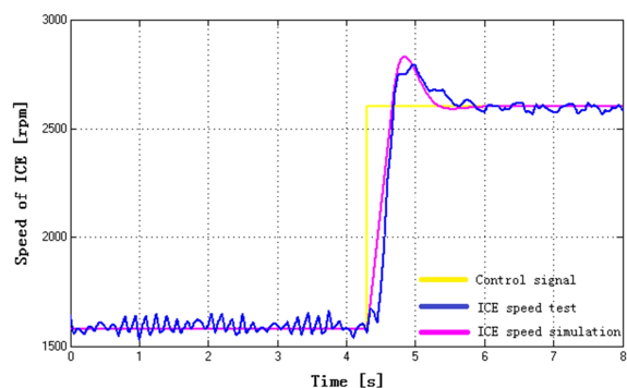
Figure 7: Step response of internal combustion engine
