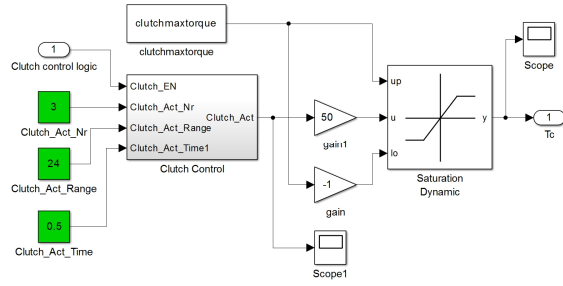
Figure 11: Simulation model of clutch current control unit
