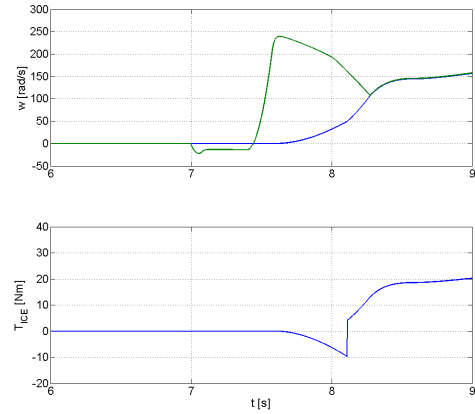
Figure 21: Simulation results of ICE speed, sun shaft speed and ICE torque during ICE starting (No10 in Table 4)
