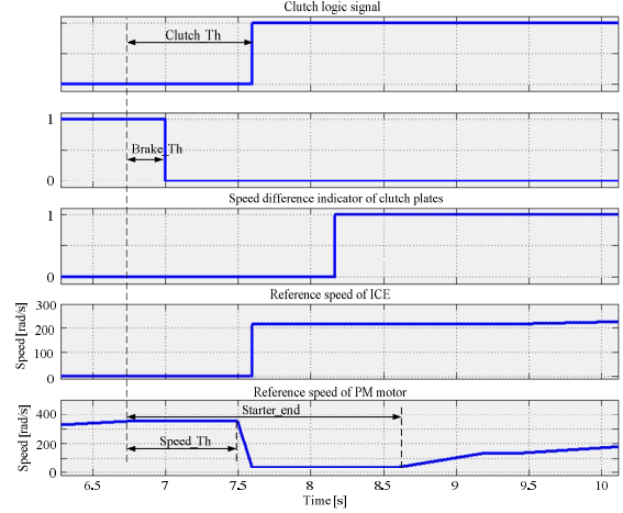
Figure 14: Indication of control signals in simulation
