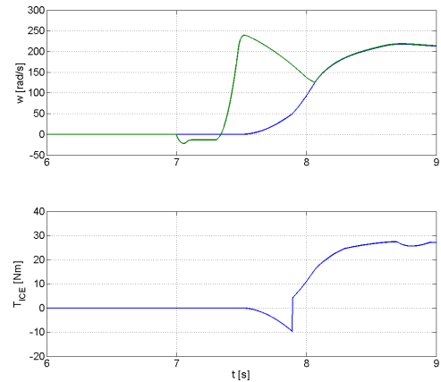
Figure 20: Simulation results of ICE speed, sun shaft speed and ICE torque during ICE starting (No6 in Table 4)
