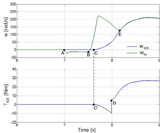
Figure 16: Simulation results of ICE speed, sun shaft speed and ICE torque during ICE starting (No3 in Table 4)
