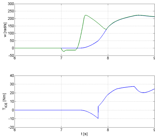
Figure 19: Simulation results of ICE speed, sun shaft speed and ICE torque during ICE starting (No5 in Table 4)
