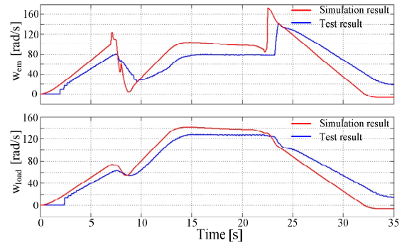
Figure 28: Simulation result and test result comparison of PM motor speed and load speed (No3 in Table 4)
