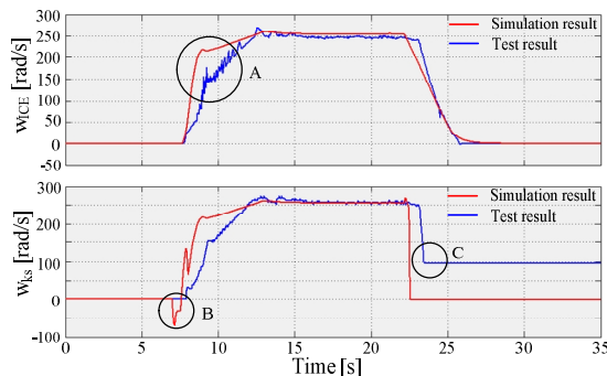
Figure 27: Simulation result and test result comparison of ICE speed and sun shaft speed (No3 in Table 4)
