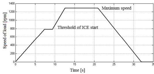
Figure 13: An exemplary driving cycle
