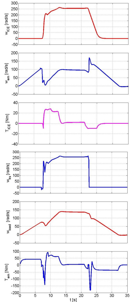
Figure 15: Simulation results for one set of parameters (No3 in Table 4)
