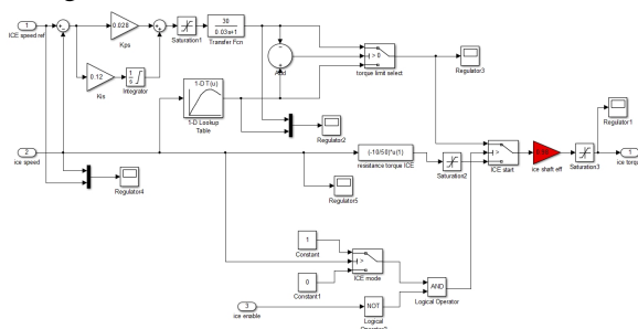
Figure 5: Simulation model of internal combustion engine
