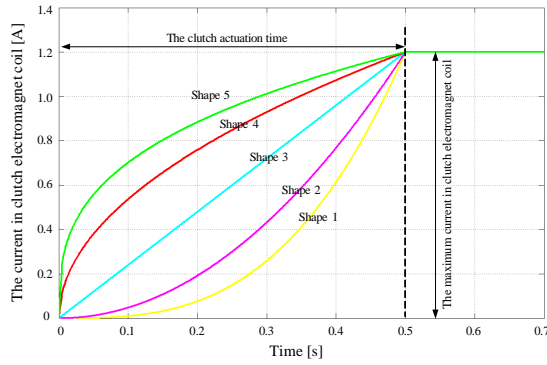
Figure 12: The control of current in clutch electromagnet coil
