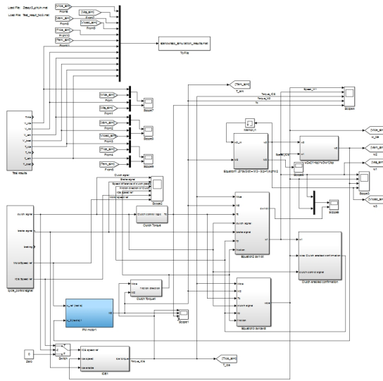
Figure 4: Simulation model of hybrid power train based on laboratory stand in MATLAB/SIMULINK environment
