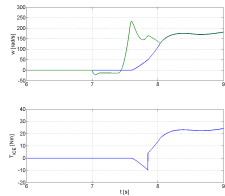
Figure 26: Simulation results of ICE speed, sun shaft speed and ICE torque during ICE starting (No16 in Table 4)
