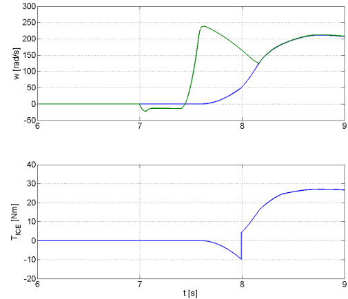
Figure 17: Simulation results of ICE speed, sun shaft speed and ICE torque during ICE starting (No2 in Table 4)
