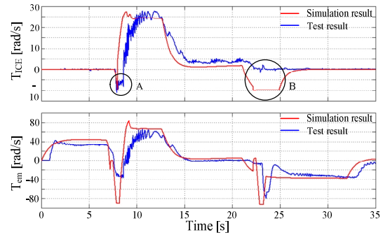
Figure 29: Simulation result and test result comparison of ICE torque and PM motor torque (No3 in Table 4)
