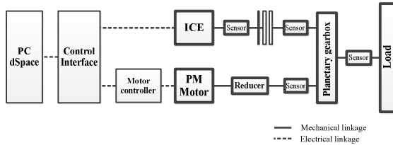
Figure 2: Configuration of hybrid power train laboratory stand according to CHPTD
