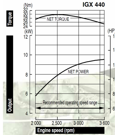
Figure 6: The external characteristic of Honda IGX440 engine
