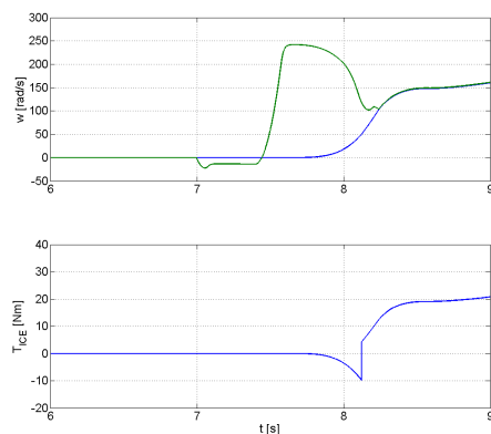
Figure 24: Simulation results of ICE speed, sun shaft speed and ICE torque during ICE starting (No13 in Table 4)
